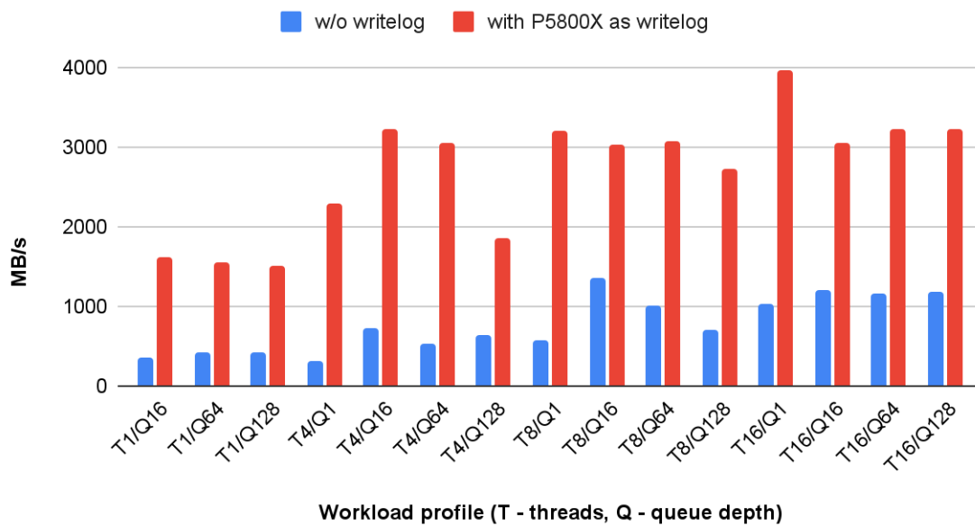
Fig. 14. Sequential write performance of a 20x single HDD zpool, with and w/o writelog.
