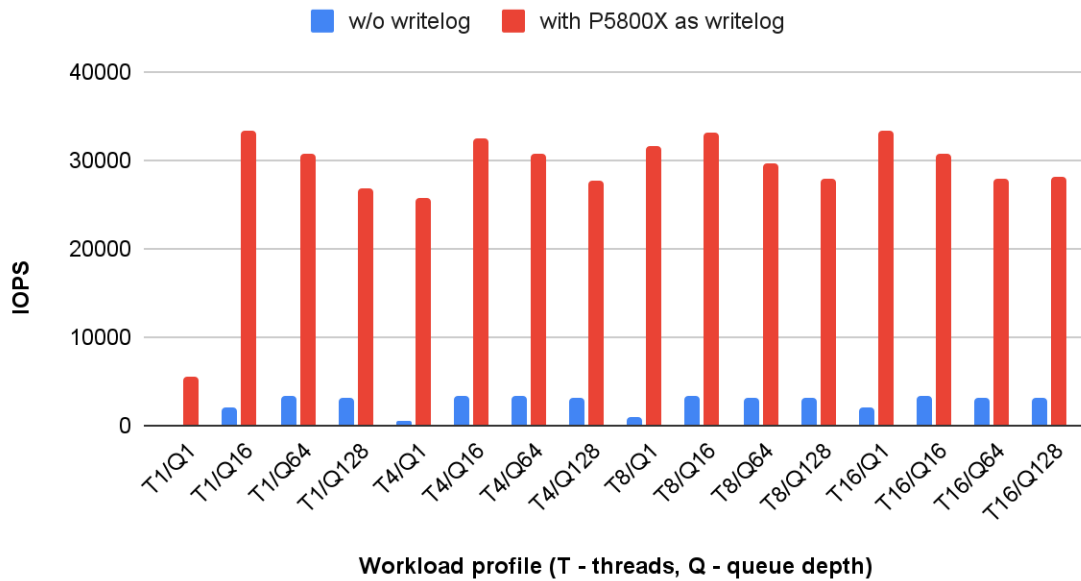
Fig. 5. Random write performance of a 10x mirror HDD zpool, with and w/o writelog.
