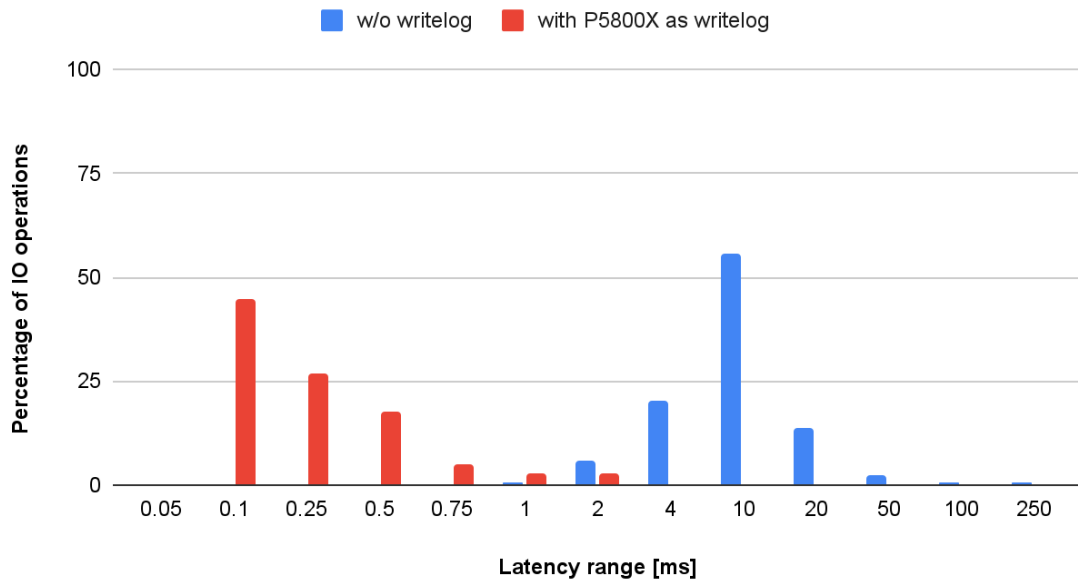
Fig. 13. Latency distribution for a random write test, done on a 20x single HDD zpool (T16/Q1), with and without writelog.
