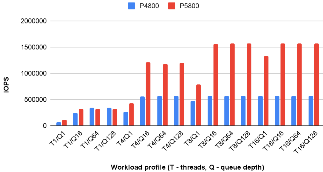
Fig. 2. Random write performance on raw device compared to P4800.
