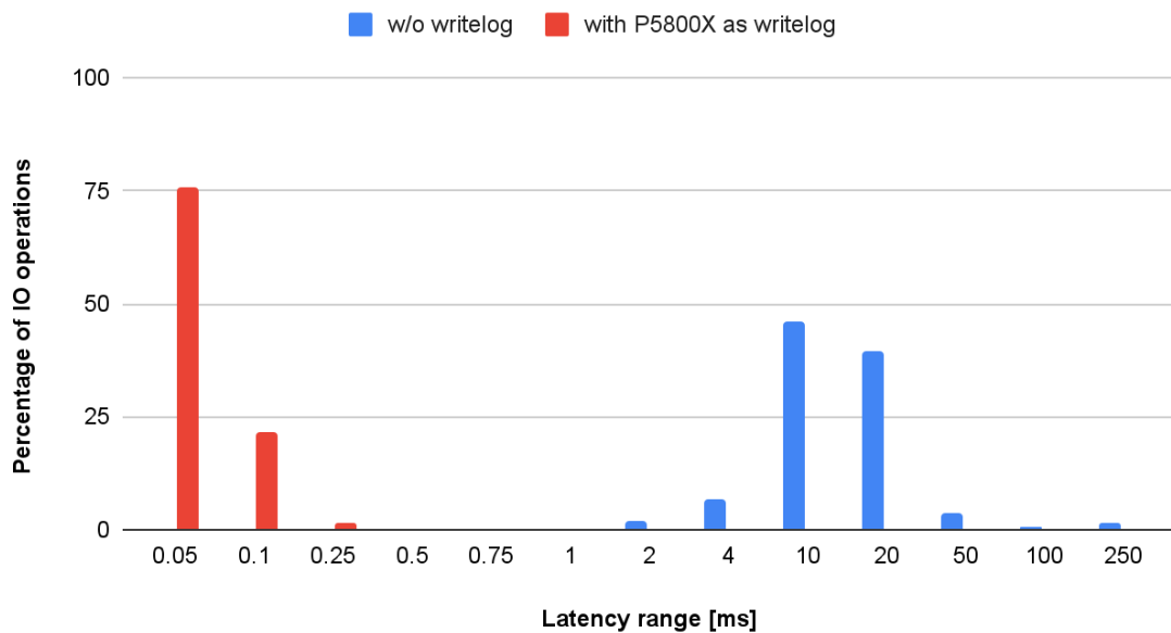
Fig. 12. Latency distribution for a random write test, done on a 20x single HDD zpool (T1/Q1), with and without writelog.
