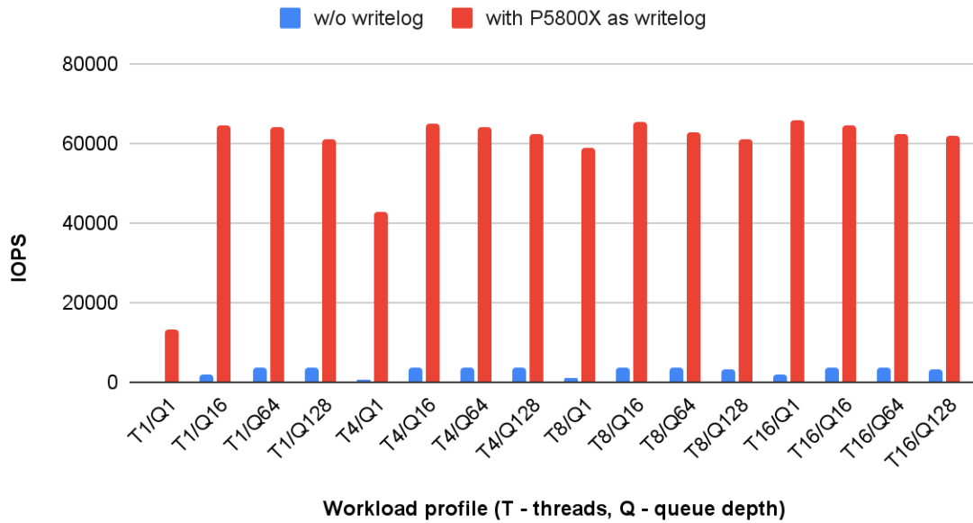
Fig. 11. Random write performance of a 20x single HDD zpool, with and w/o writelog.
