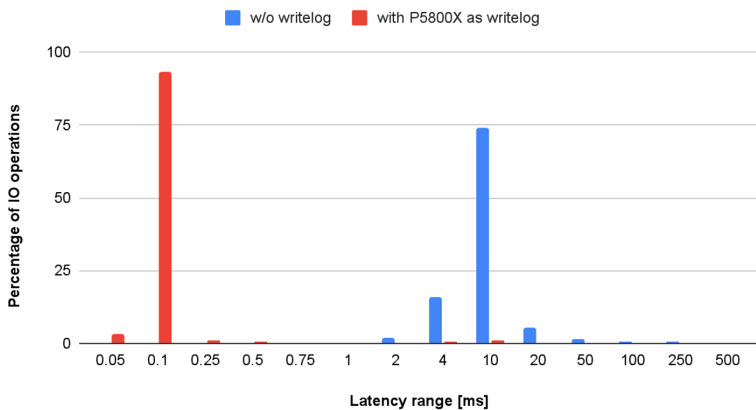
Fig. 6. Latency distribution for a random write test, done on a 10x mirror HDD zpool (T1/Q1), with and without writelog.
